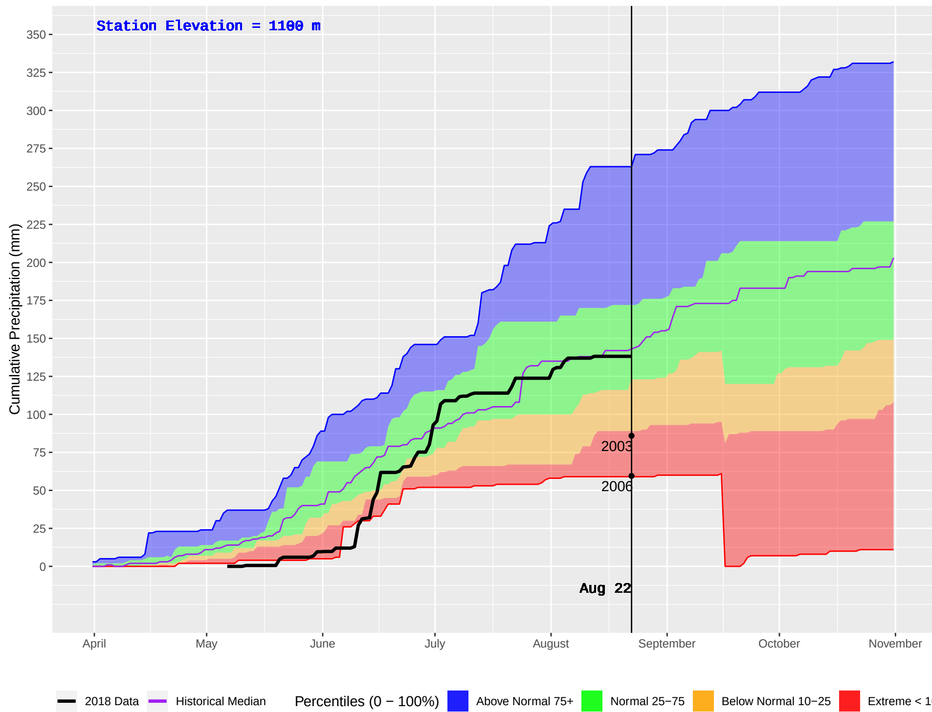
CHURN CREEK (832) : Historical (2003–2016) and Current (2018) Daily Cumulative Precipitation
